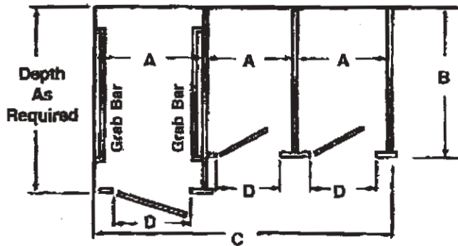
Typical Toilet Partition Layout
